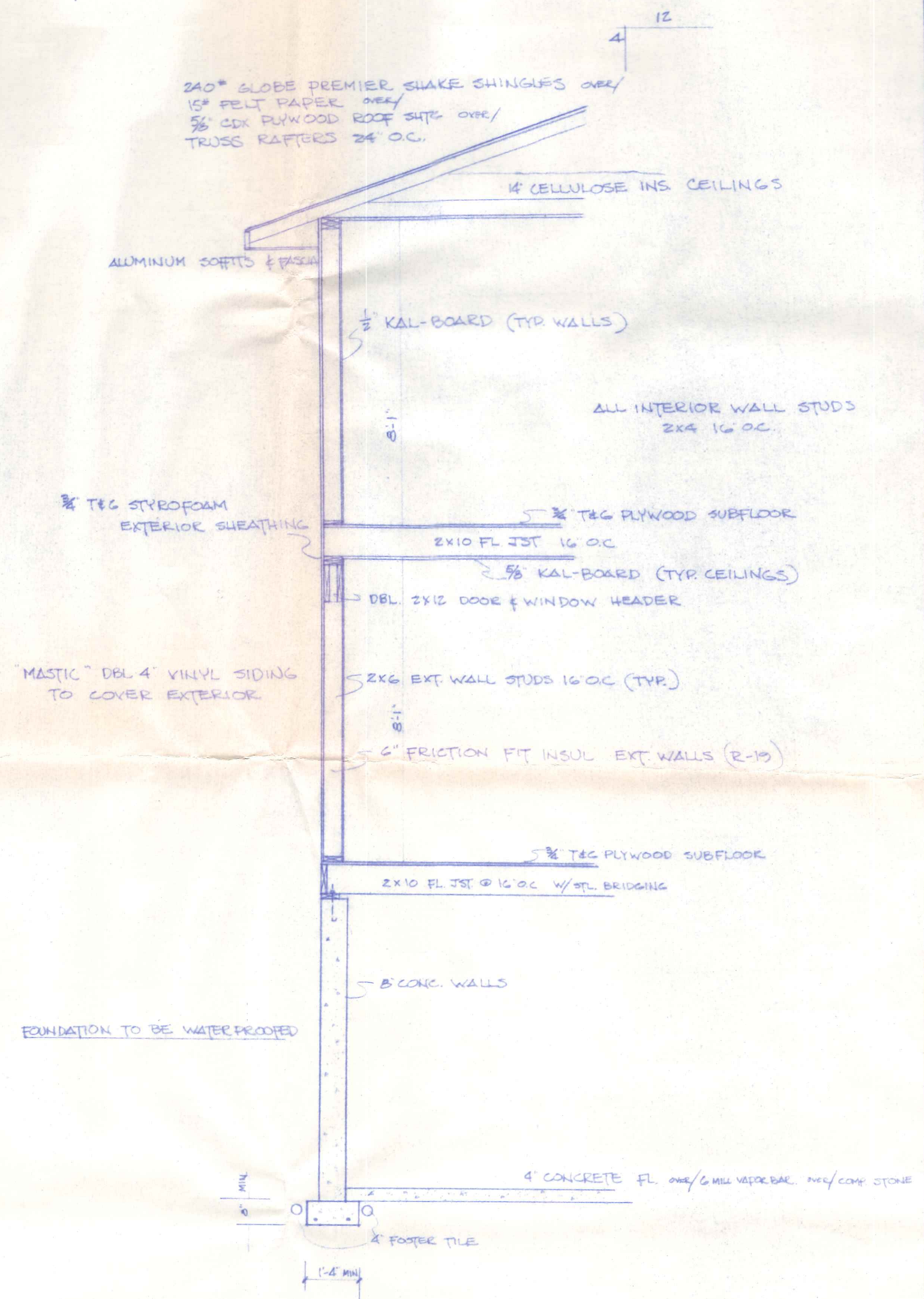
TYPICAL WALL SECTION
