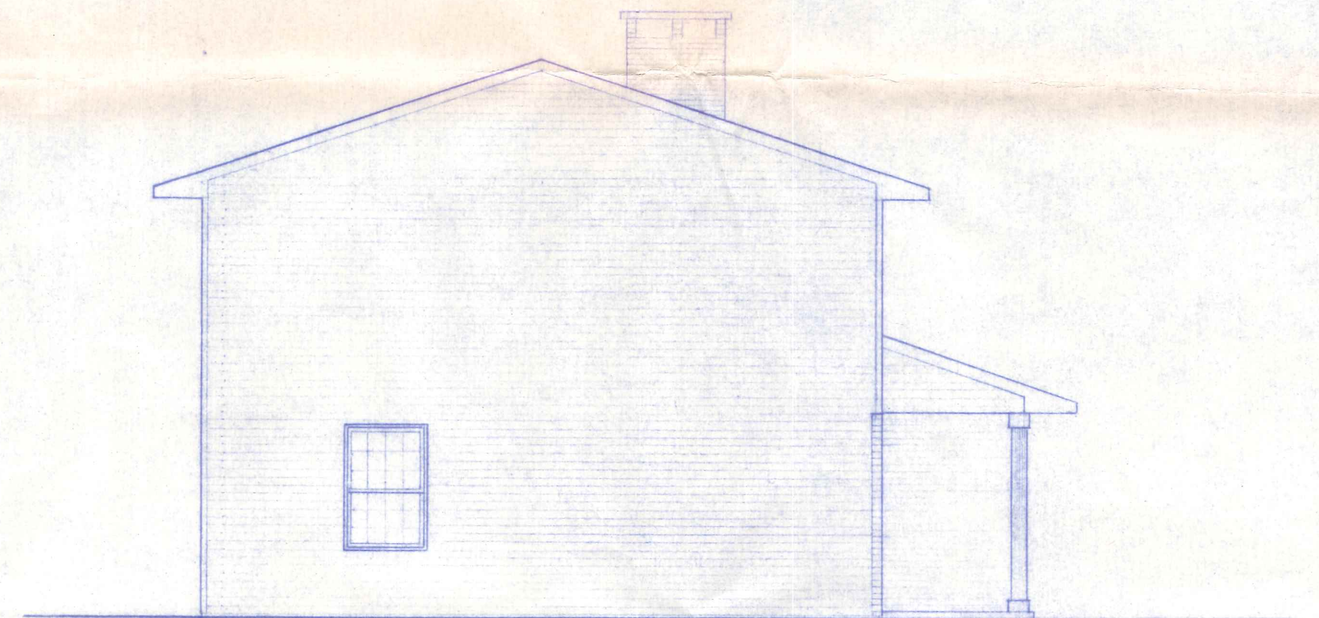
EAST ELEVATION
