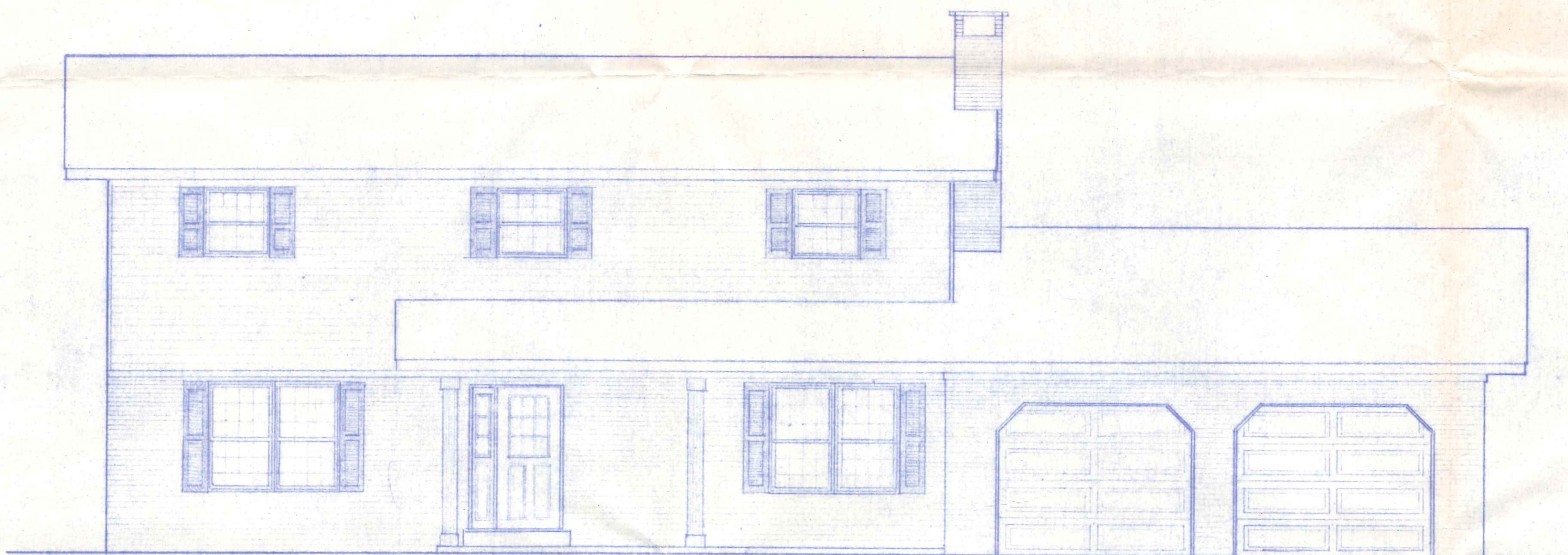
NORTH ELEVATION
