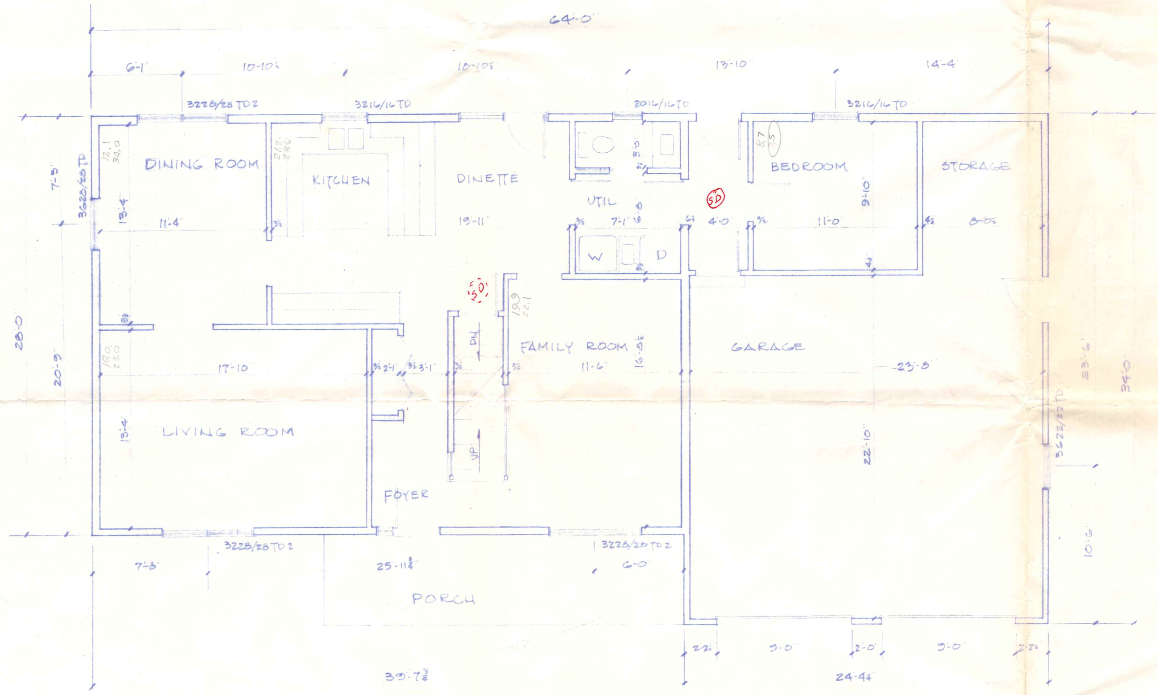
1 st FL. - FLOOR PLAN SCALE 1/8"=1'-0"
